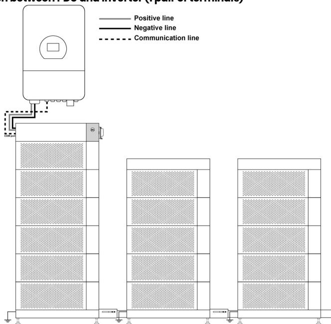
Connection between PDU and inverter (2 pairs of terminals)
